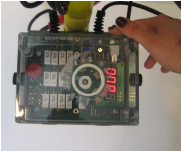
Unit is equipped with 1500VDC surge suppression and push button voltage meter
